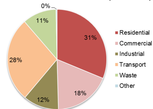
Breakdown of aggregate Community GHG Inventories of 4 cities as of 2007 (28M tCO 2 e)
